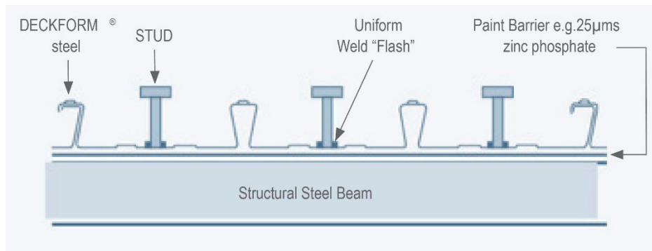
Figure 1. Schematic of steel composite decking incorporating DECKFORM® steel
