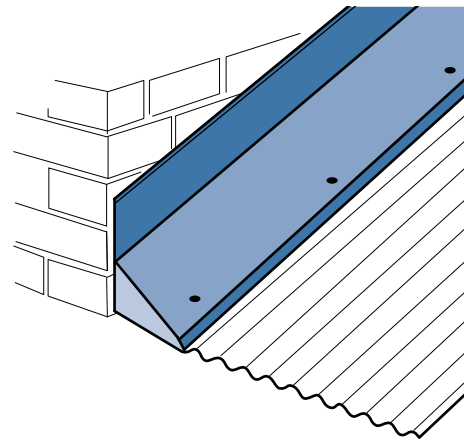
Figure 3.2.3 Angled apron 45°.
