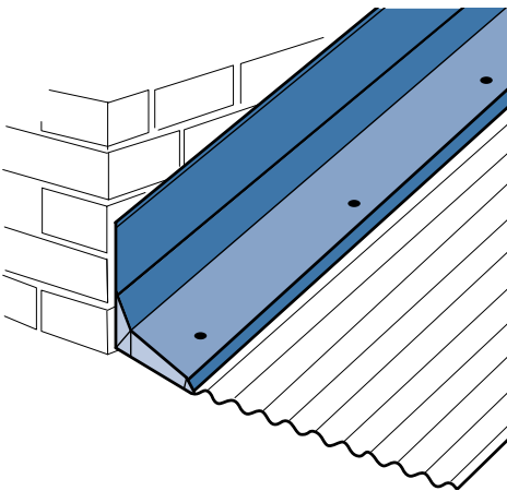
Figure 3.2.5 Angled apron 110°.
