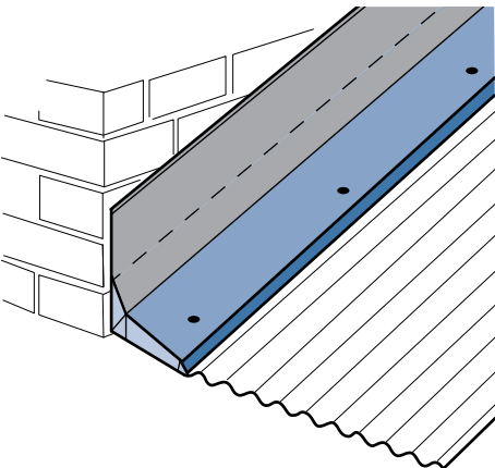
Figure 3.2.6 Two piece apron.
