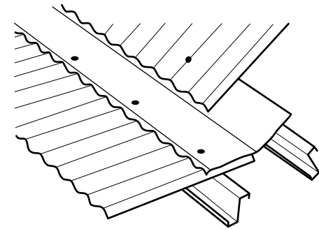
Flashing at change of pitch
