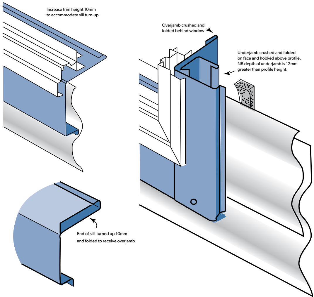
Figure 4.14.3 Flush window sill flashing.
