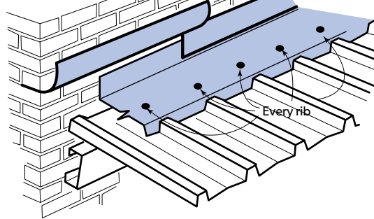
Parapet Flashing
