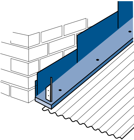
Figure 3.2.2 Angle diverter.
