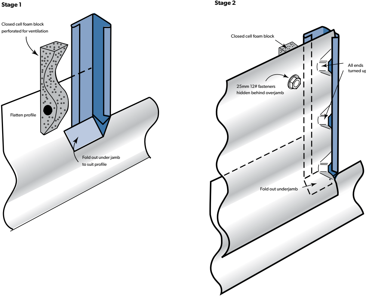
Figure 4.14.1 Flush window flashings.
