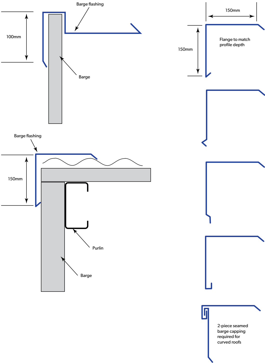
Figure 3.18.1 Barge gutters and cappings.
