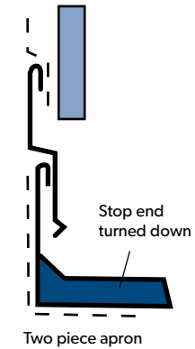
Two piece apron
