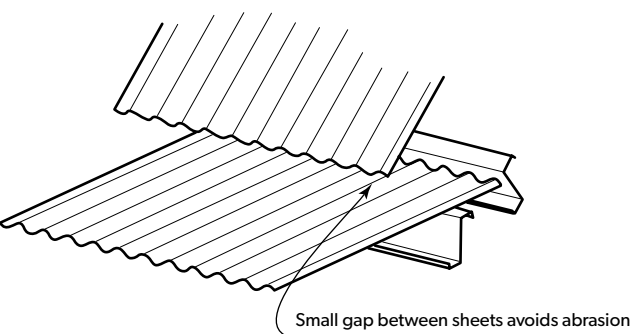
Change of pitch without flashing
