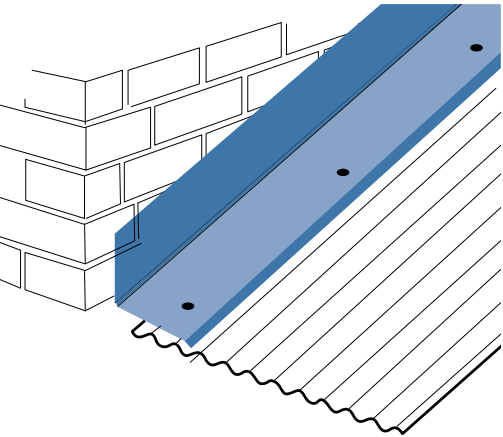
Figure 3.2.1 Chased apron.
