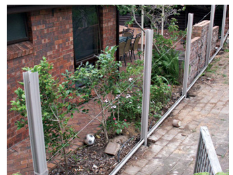
Set all the bottom rails into position ensuring a 50mm ground clearance.
