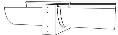
LYSAGHT® Commercial Half Round gutter with A4 External Bracket
