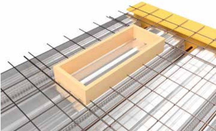
Max 400mm x 1000mm small penetrations not cutting SlimDek 210® ribs with timber form breakout
