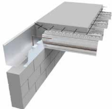
SlimDek 210® perpendicular to wall with cantilever edge form
