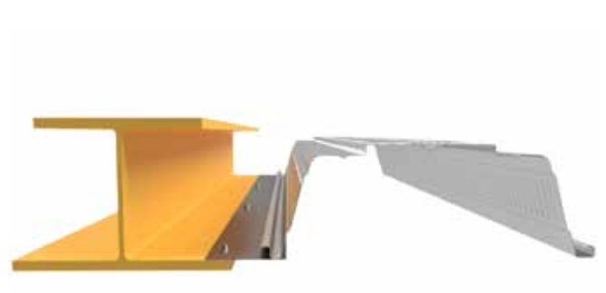
Edge beam with edge form SlimDek 210® full sheet parallel to beam with closure plate
