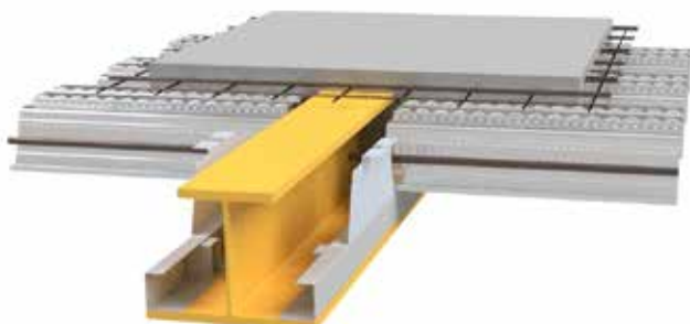
SlimFlor® beam cold formed packer details
