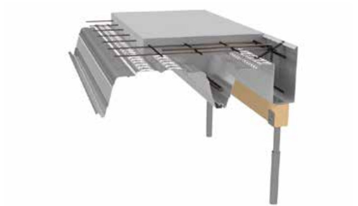
Unsupported edge detail ripped sheet with closure flashing and edge form - propping required
