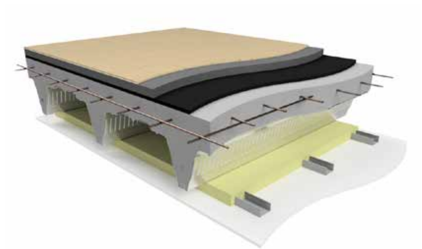
Tiled floor wet area with insulation
