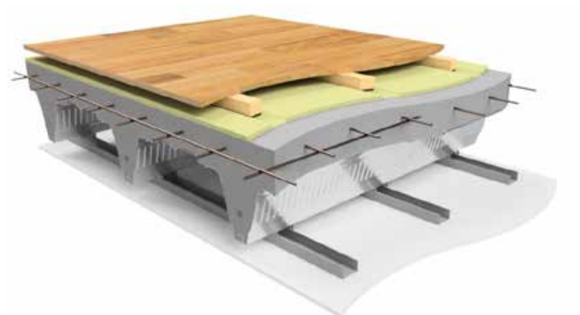
Battened layered resilient floor
