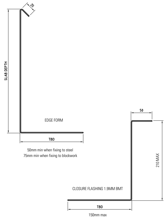
Figure 9 SlimDek 210® Edge Form and Closure Flashing Dimensions
