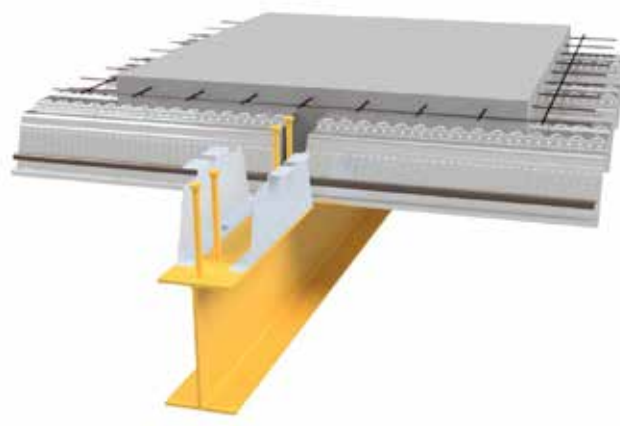
Figure 19 Internal Down-stand Beam
