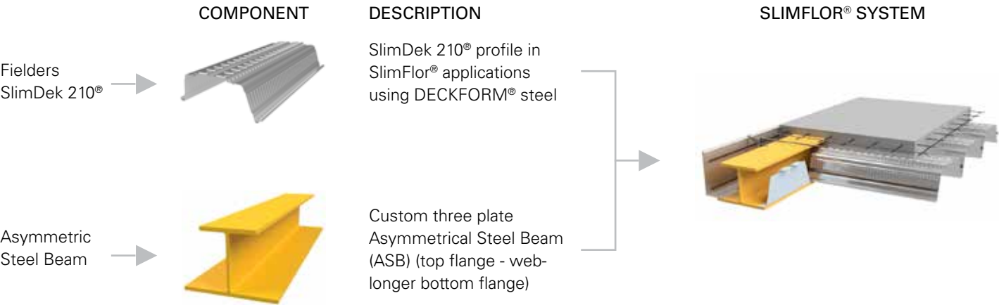
Figure 1 SlimFlor® System
