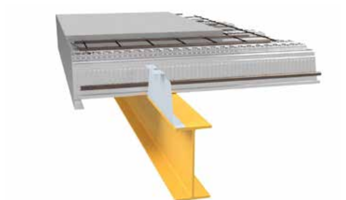
Downstand beam edge detail with cantilever
