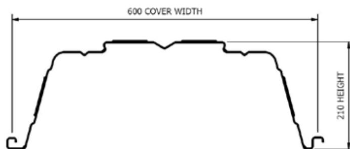
Figure 2 SlimDek 210® Section
