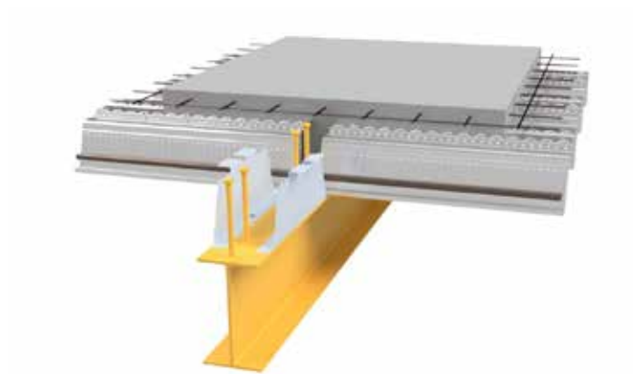
Downstand beam with SlimDek 210® composite slab continuous
