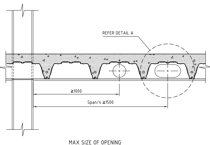
Figure 24 Web Penetration Rules
