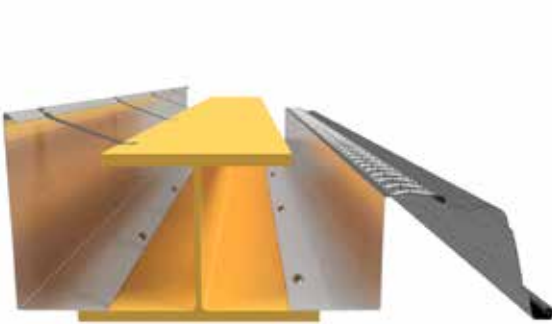
Edge beam with edge form SlimDek 210® cut along its length with closure flashing
