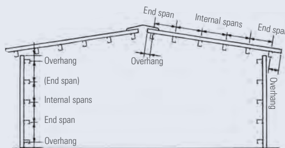
Figure 2: Span Locations
