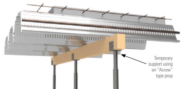
PROPPING OF SLIMDEK 210™
