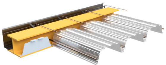
FIXING OF SLIMDEK 210™
