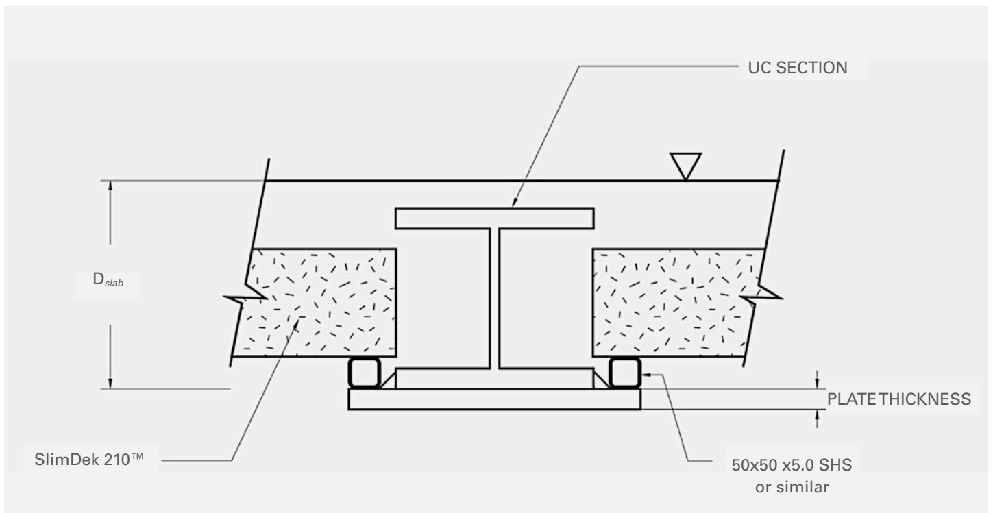
Figure F.3.5.4 Dimensions of CUSTOM ASB
