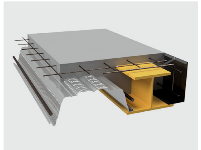
Figure F3.5.1 Fielders SlimFlor®
