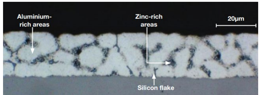
Figure 1a: ZINCALUME® steel AZ150 (superseded)
