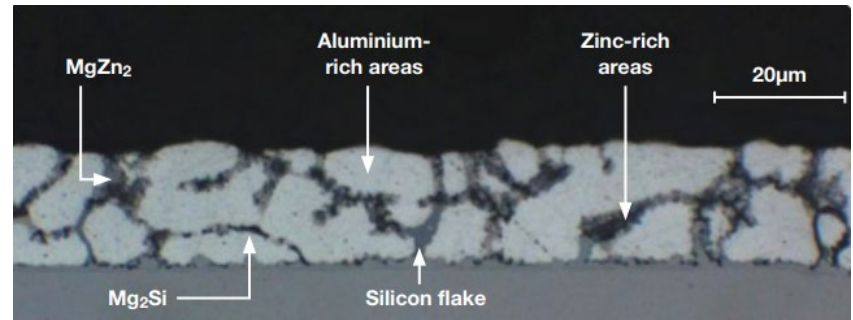
Figure 1b: Next generation ZINCALUME® steel AM125
